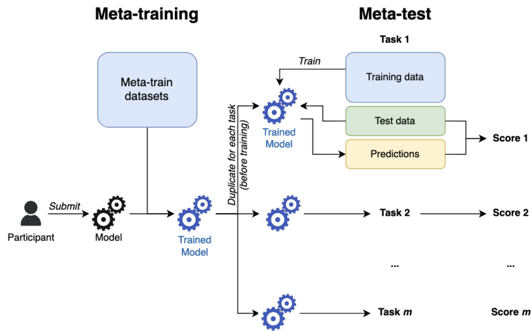
Figure 3: Meta-learning evaluation workflow. The submitted model is trained on meta-train datasets, and then it is tested on a set of meta-test tasks.
