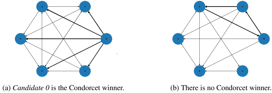
Figure 10: Condorcet graphs where vertices represents candidates, and where there is an arrow between candidates \mathbf{u} and \mathbf{v} if \mathbf{u} is more frequently better than \mathbf{v} according to the judges' preferences. In the left example, Candidate 0 is a clear Condorcet winner, beating all other candidates. The right example exhibit a Condorcet paradox, as Candidate 0 beats Candidate 1 , Candidate 1 beats Candidate 2 and Candidate 2 beats Candidate 0 , resulting in a cycle. Bold arrows are highlighted for clarity.
